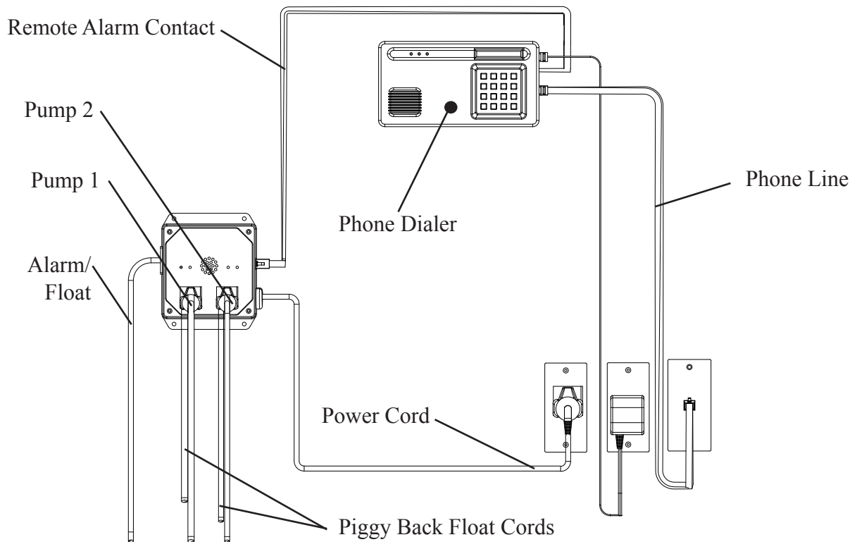
Pump Guard and Dialer Install Setup
