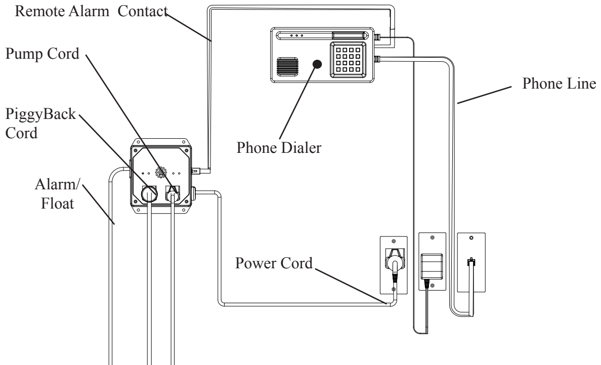
Pump Guard and Dialer Install Setup
